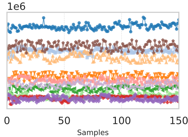
cycle_activity.cycles_mem_any
